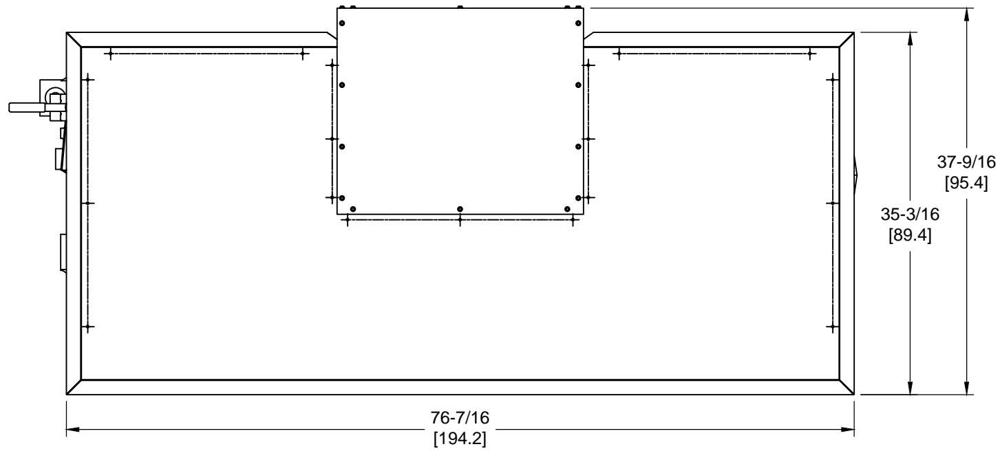
OUTDOOR TOP VIEW
